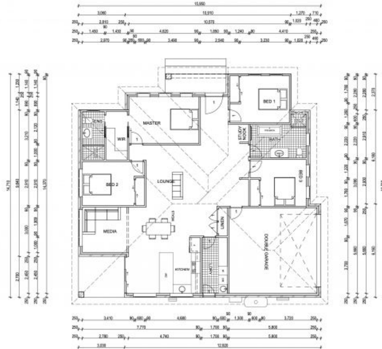
1. GROUND FLOOR 1:100
